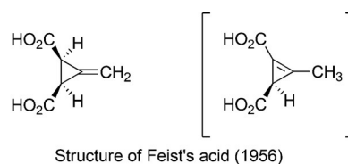
Structure of Feist's acid (1956)
